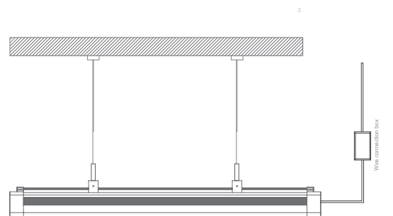
B: Install the steel cable holder to ceiling
