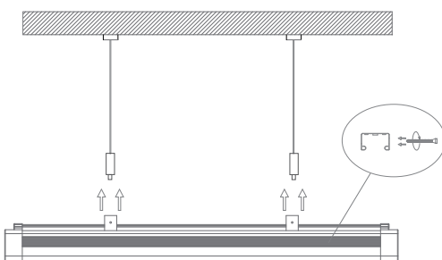
C : Install the fixture to the steel cable
