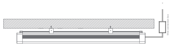
B: Install the clipsto the ceiling
