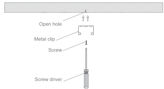
B: Install the clipsto the ceiling
