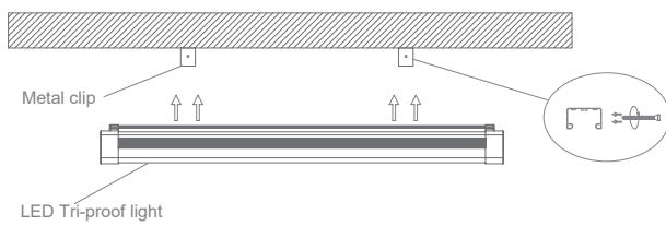
C: Install the lamp according to the clips`
